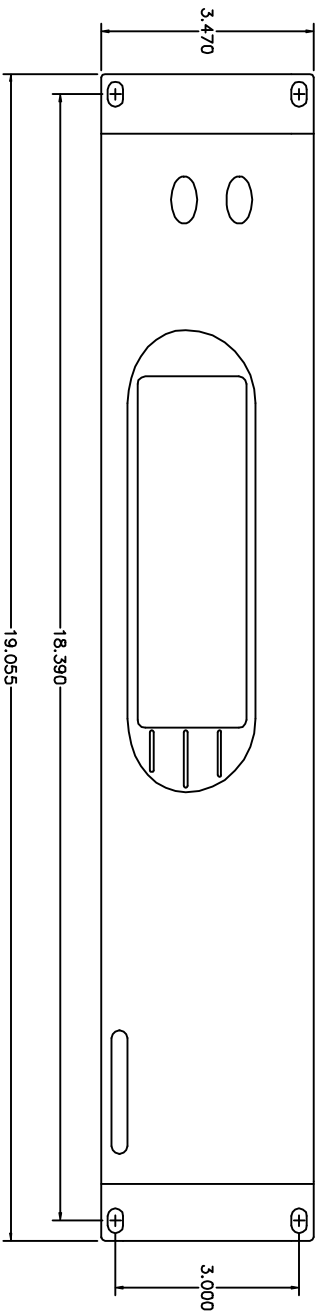
FRONT VIEW RACK MOUNT DIMENSIONS
