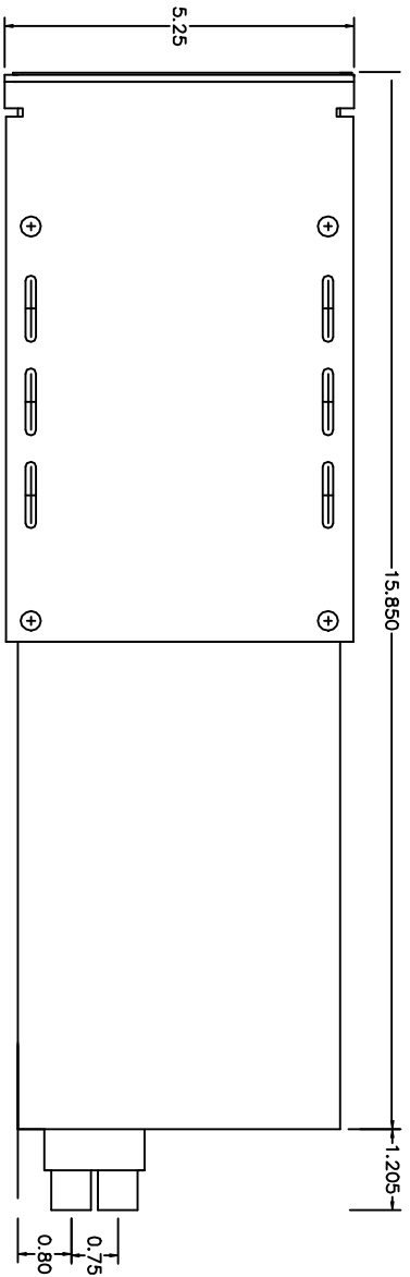
Rack Mount Brackets Part No. 7831950
